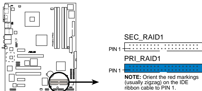
P5GD2 PRO RAID connectors
