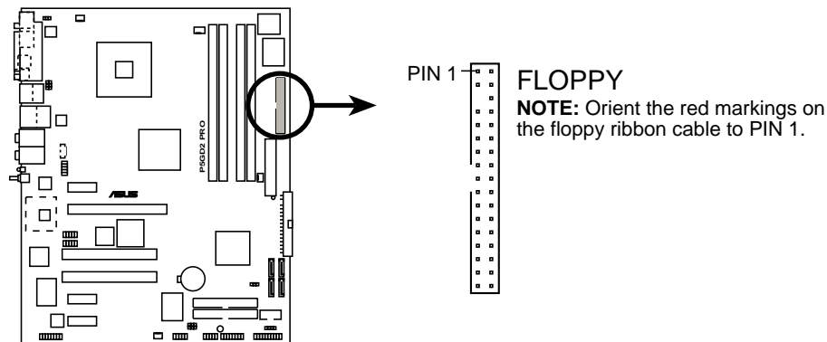
P5GD2 PRO Floppy disk drive connector
