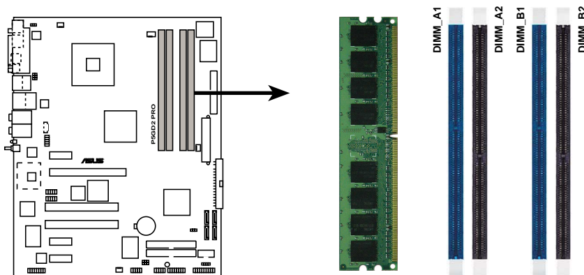
P5GD2 PRO 184-Pin DDR DIMM sockets
