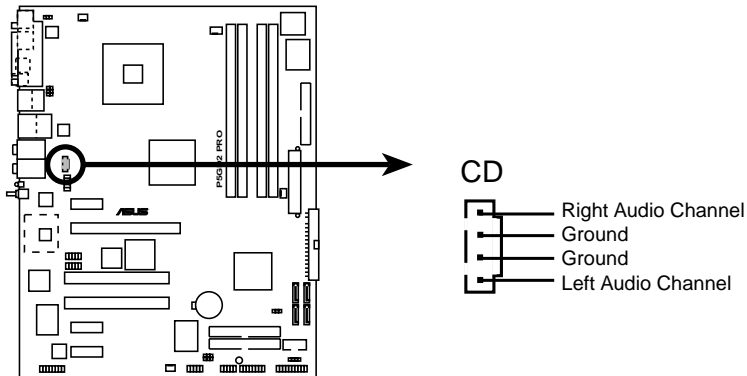
P5GD2 PRO CD audio connector
