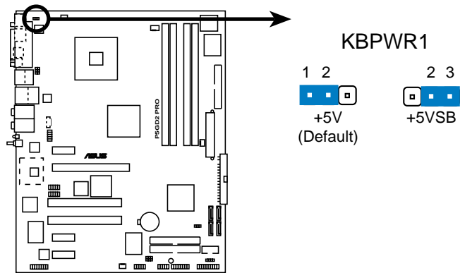
P5GD2 PRO Keyboard power setting
